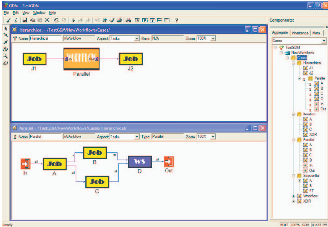
Figure 5. Inner Workflow. Parallel is an inner workflow that is embedded into a sequential workflow.
