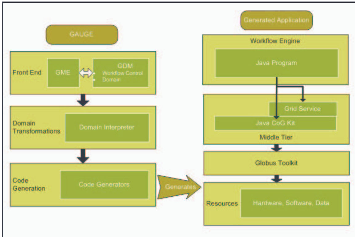
Figure 2. Architecture of the Modeling Environment. The left side of the figure presents the architecture for GAUGE. The right side presents the organization of the programs generated by GAUGE.
