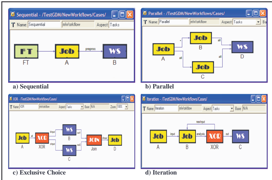
Figure 4. Control constructs supported by GAUGE. a) Sequential execution of tasks. b) AND-Split & Join, both B and C are executed after A. D is executed after B and C have completed their execution. c) XOR-Split & Join. After completion of A, either B or C is executed (but not both). D is executed after the completion of B or C. d) B can be executed many times until the condition in the XOR routes the flow to C.
