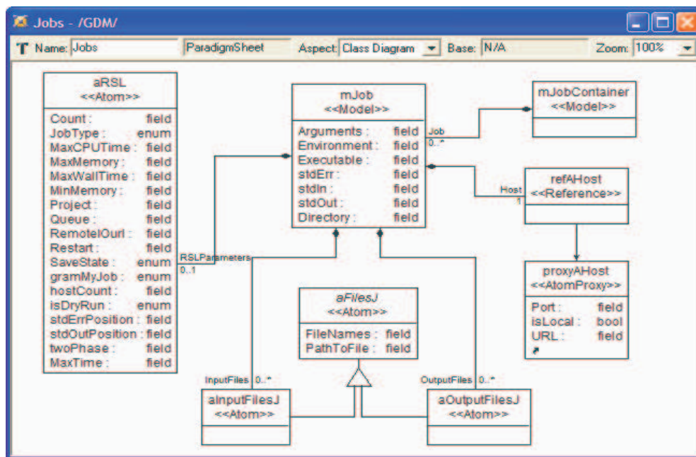
Figure 3. GDM language specification for job tasks. This figure presents the manner in which the relation of the different (GME) classes specify a construct in GDM.
